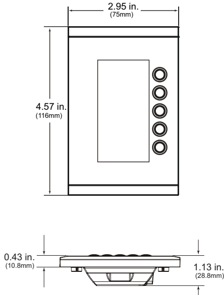
Figure 2: Saturn DLT Keypad Dimensions
