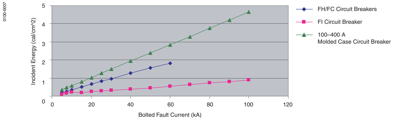
Figure 7: Incident Energy vs. Bolted Fault Current for 100 A Circuit Breakers—Simplified Equations vs. Actual Data
