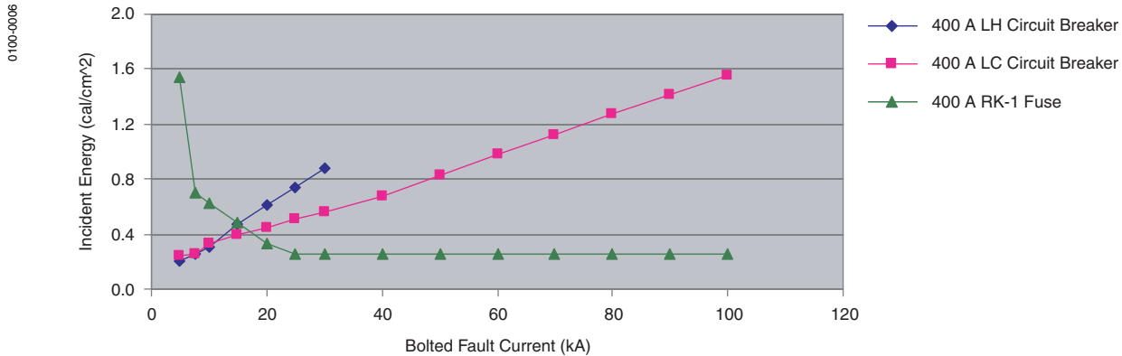
Figure 6: Incident Energy vs. Bolted Fault Current for 400 A Circuit Breakers and 400 A Class RK-1 Fuses
