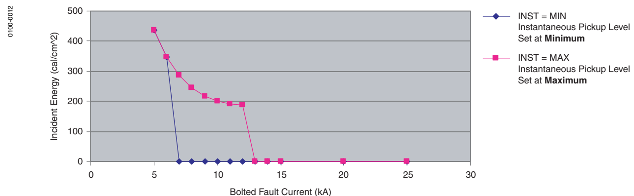
Figure 12: Incident Energy vs. Bolted Fault Current for 600 A LI Circuit Breakers
