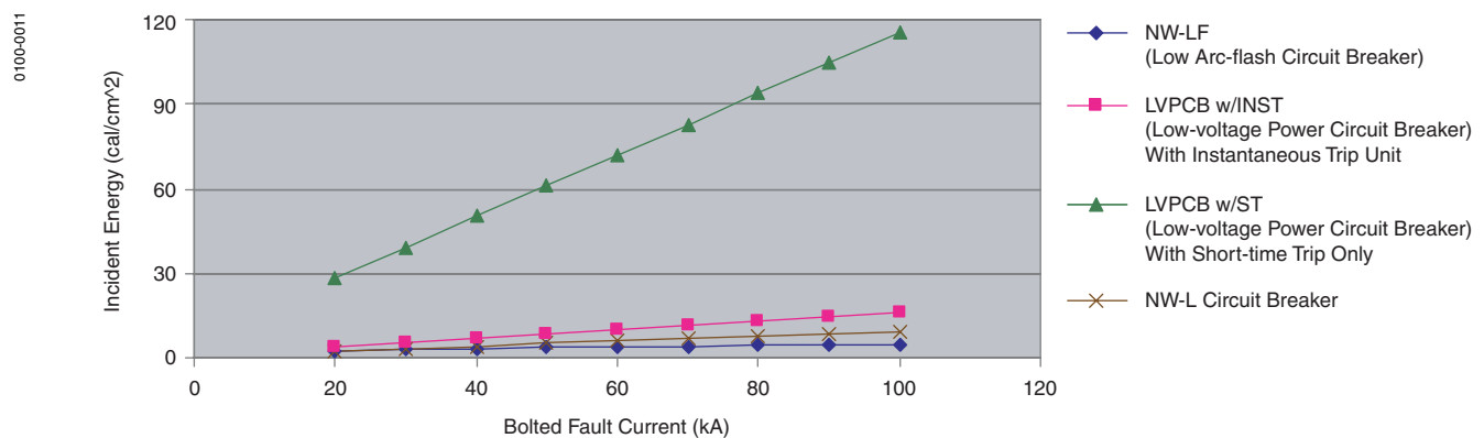
Figure 11: Incident Energy vs. Bolted Fault Current for 2000 A Circuit Breakers—Simplified Equations vs. Actual Data
