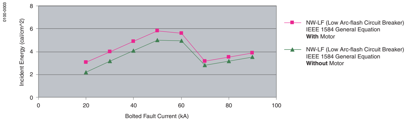
Figure 3: Incident Energy Levels vs. Bolted Fault Current at MCC, With and Without Motor Contribution
